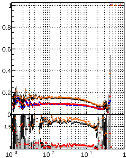
Fake rate vs \sqrt{s} DQM Displaced SUSY CKEFit DQM Displaced SUSY CKEFit_BDT DQM Displaced SUSY mkFit_BDT
