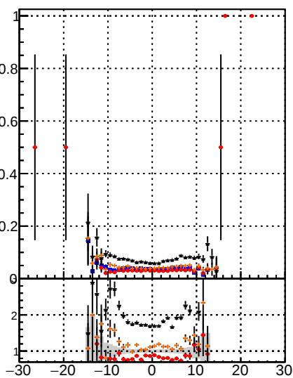
Fake rate vs d BDT Displaced SUSY CKF BDT Displaced SUSY CKF+BDT BDT Displaced SUSY CKF+BDT
