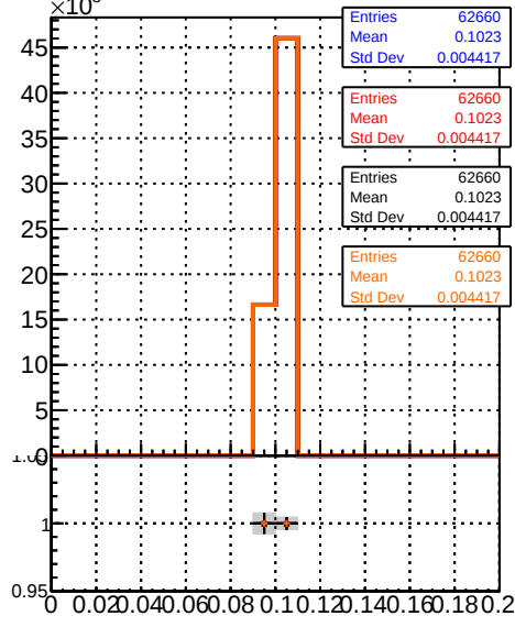
GeneratedAIV_Z Legend: DQM_DisplacedSUSY CKF (blue line), DQM_DisplacedSUSY mkFit (red line), DQM_DisplacedSUSY CKF BDT (black line), DQM_DisplacedSUSY mkFit BDT (orange line)
