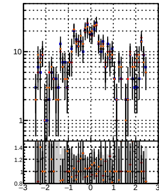
SUSY — CKE SUSY — mKE fit SUSY — CKE BDT SUSY — mKE fit BDT
