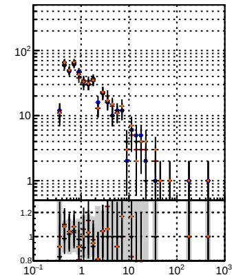
SUSY — CKE SUSY — mKE fit SUSY — CKE BDT SUSY — mKE fit BDT
