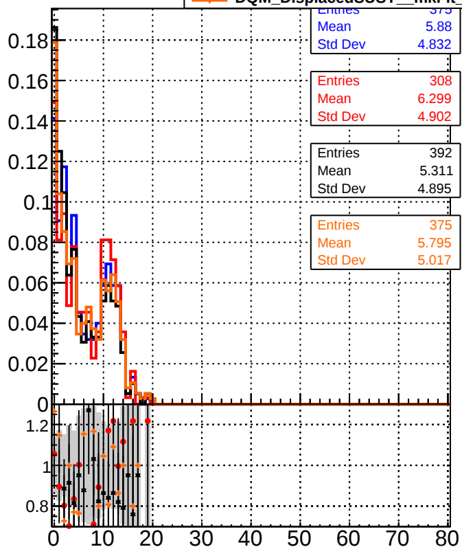
Legend for the bottom row of plots: DQM_DisplacedSUSY_CKF_ (Blue line with squares) DQM_DisplacedSUSY_mkFit_ (Red line with circles) DQM_DisplacedSUSY_CKF_BDT_ (Black line with crosses) DQM_DisplacedSUSY_mkFit_BDT_ (Orange line with crosses)
