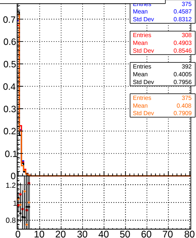
Legend for the bottom row of plots: DQM_DisplacedSUSY_CKF_ (Blue line with squares) DQM_DisplacedSUSY_mkFit_ (Red line with circles) DQM_DisplacedSUSY_CKF_BDT_ (Black line with crosses) DQM_DisplacedSUSY_mkFit_BDT_ (Orange line with crosses)
