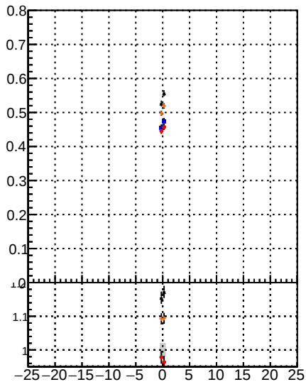
Fake rate vs d BSM Displaced SUSY CKFit BDT BSM Displaced SUSY CKFit BDT BSM Displaced SUSY CKFit BDT
