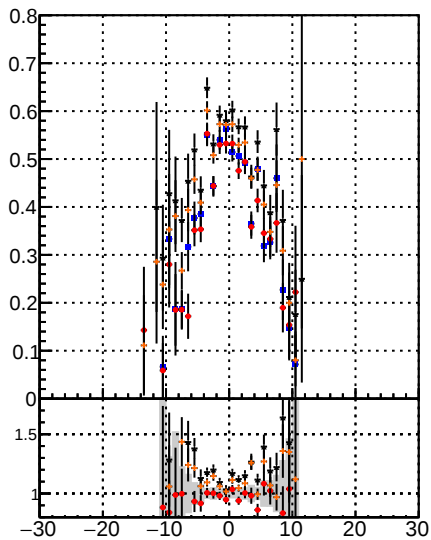
Fake rate vs d BSM Displaced SUSY CKFit BDT BSM Displaced SUSY CKFit BDT BSM Displaced SUSY CKFit BDT
