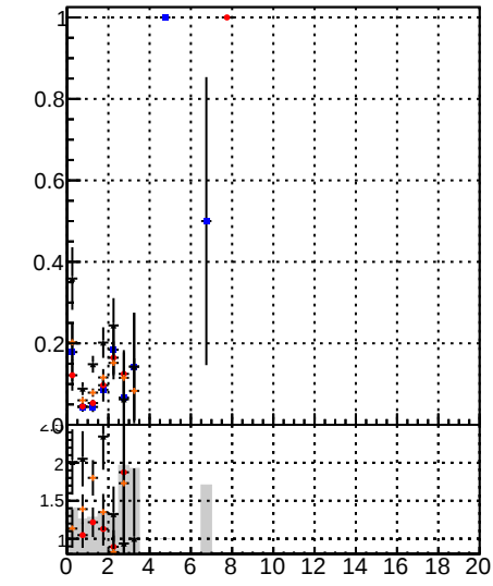
Fake rate vs. \chi^2 for BDT, Displaced SUSY, and CKFit
