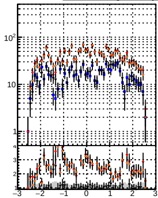
N of reco track vs e
