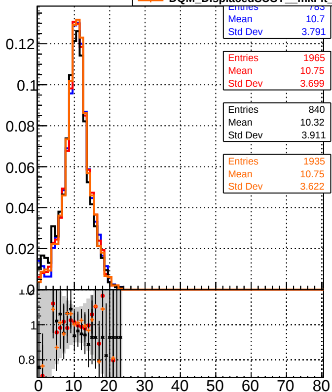
— DQM_DisplacedSUSY_CKF_ (Blue) — DQM_DisplacedSUSY_mkFit_ (Red) — DQM_DisplacedSUSY_CKF_BDT_ (Black) — DQM_DisplacedSUSY_mkFit_BDT_ (Orange)
