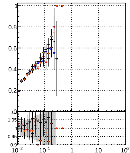
DOM Displaced SUSY CKE Fit DOM Displaced SUSY CKE Fit BDT DOM Displaced SUSY mkFit BDT
