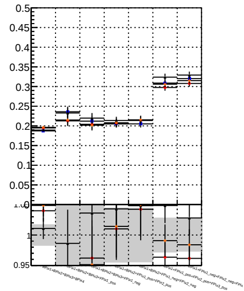
Fake rate vs. BSM Displaced SUSY CKFit CKFit_BDT BSM Displaced SUSY CKFit CKFit_BDT BSM Displaced SUSY CKFit CKFit_BDT
