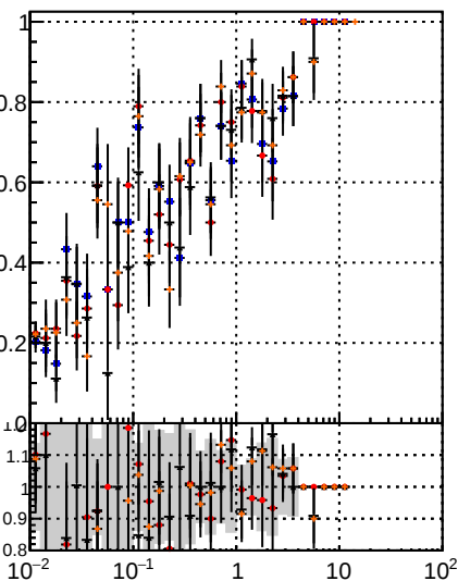
DOM Displaced SUSY CKE DOM Displaced SUSY CKE fit DOM Displaced SUSY mkt fit BDT DOM Displaced SUSY mkt fit BDT
