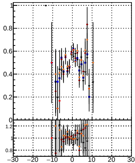
DOM Displaced SUSY CKE DOM Displaced SUSY CKE fit DOM Displaced SUSY mkt fit BDT DOM Displaced SUSY mkt fit BDT
