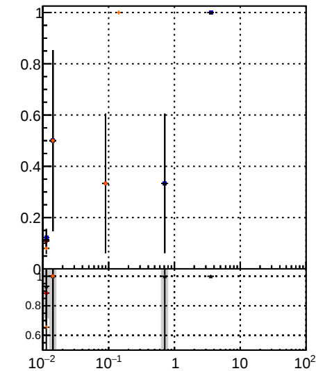
Fake rate vs vertpos Legend: DOM (blue) Displaced SUSY (orange) CKE (red) BDT (black) DOM (blue) Displaced SUSY (orange) CKE (red) BDT (black) DOM (blue) Displaced SUSY (orange) CKE (red) BDT (black)
