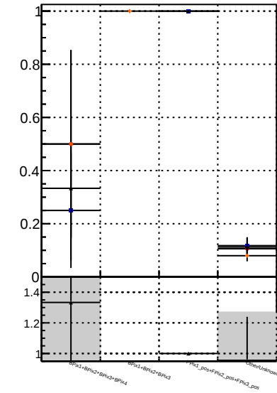
Fake rate vs. BSM Displaced SUSY BSM Displaced SUSY CKFit BSM Displaced SUSY CKFit_BDT BSM Displaced SUSY BSM Displaced SUSY CKFit BSM Displaced SUSY CKFit_BDT BSM Displaced SUSY BSM Displaced SUSY CKFit BSM Displaced SUSY CKFit_BDT
