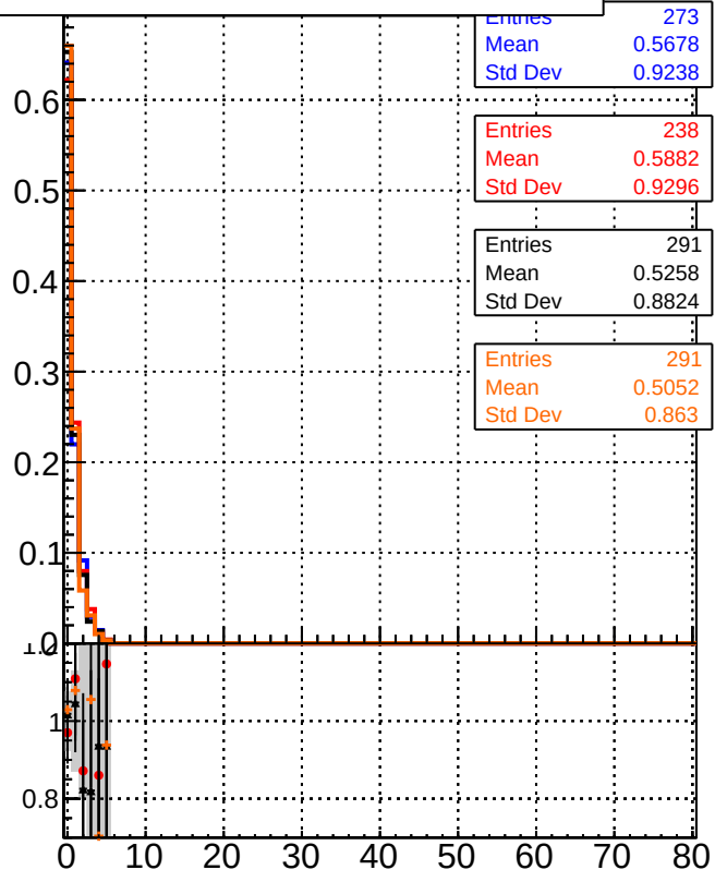
Legend for the bottom row of plots: —■— DQM_DisplacedSUSY_CKF —●— DQM_DisplacedSUSY_mkFit —■— DQM_DisplacedSUSY_CKF_BDT —■— DQM_DisplacedSUSY_mkFit_BDT
