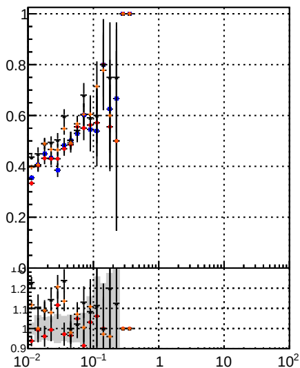
Fake rate vs v —●— DOM Displaced SUSY CKE —●— DOM Displaced SUSY CKE Fit —●— DOM Displaced SUSY CKE Fit BDT —●— DOM Displaced SUSY mkFit BDT
