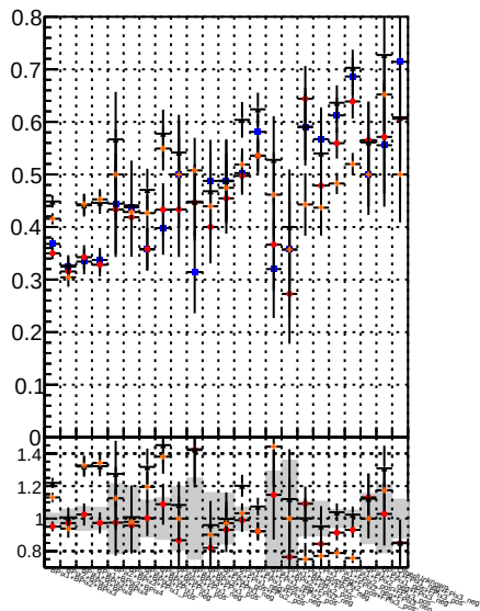
Fake rate vs. \chi^2 for BSM, Displaced, SUSY, CKF, CKFit, BDT, and CKFit+BDT
