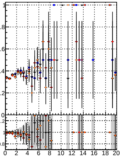
Fake rate vs. DOM Displaced SUSY CKF CKFit BDT DOM Displaced SUSY CKF CKFit BDT
