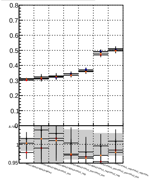
Fake rate vs. DOM Displaced SUSY CKF CKFit BDT DOM Displaced SUSY CKF CKFit BDT
