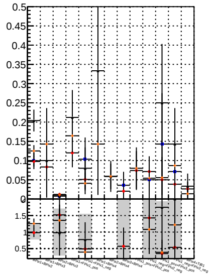
Fake rate vs. BDM Displaced SUSY CKE Fit BDT
