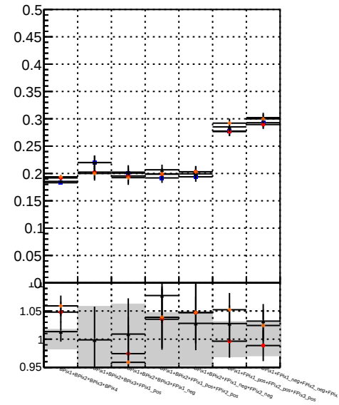
Fake rate vs. BSM Displaced SUSY CKE BSM Displaced SUSY CKE fit BSM Displaced SUSY CKE fit BDT BSM Displaced SUSY CKE fit BDT
