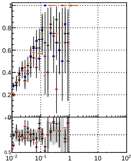
Fake rate vs vertpos DOM Displaced SUSY CKE DOM Displaced SUSY CKEfit DOM Displaced SUSY mktFit BDT
