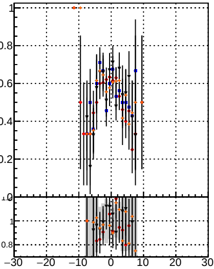
Fake rate vs vertpos Legend: DOM Displaced SUSY CKE DOM Displaced SUSY CKE fit DOM Displaced SUSY mkFit BDT
