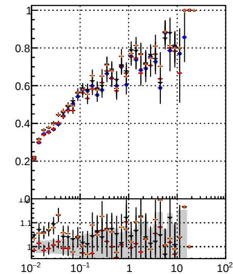
DOM Displaced SUSY CKE DOM Displaced SUSY CKEfit DOM Displaced SUSY BDT DOM Displaced SUSY mktfit BDT
