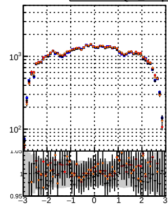
N of reco track vs \eta BQM Displaced SUSY GKE-fit BDT BQM Displaced SUSY MKF-fit BDT
