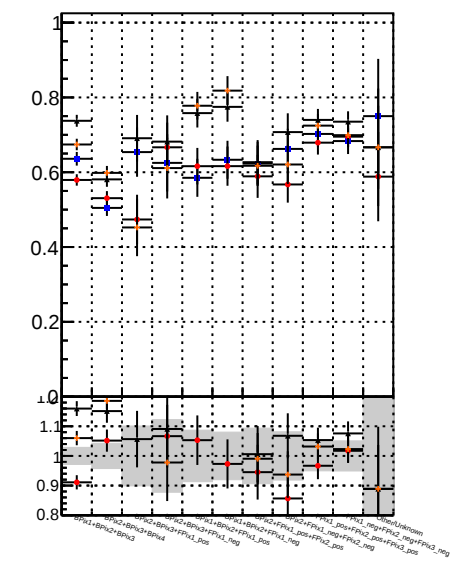
Fake rate vs. BSM Displaced SUSY CKFit BDT BSM Displaced SUSY CKFit BDT BSM Displaced SUSY CKFit BDT
