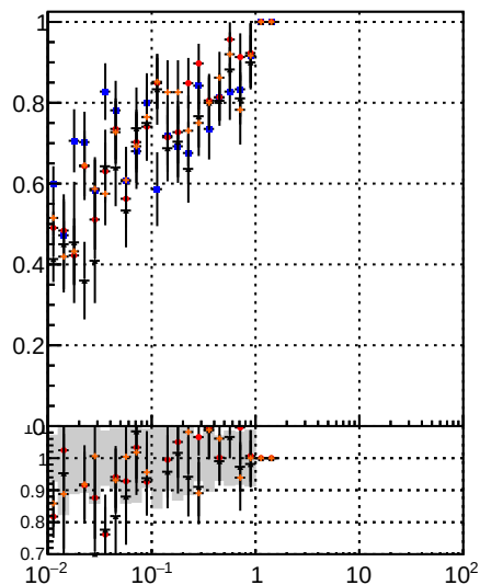
Fake rate vs v DOM Displaced SUSY CKE DOM Displaced SUSY CKEfit DOM Displaced SUSY CKEfit BDT
