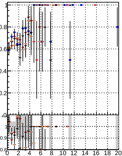
Fake rate vs. BSM Displaced SUSY CKFit CKFit_BDT BSM Displaced SUSY CKFit CKFit_BDT BSM Displaced SUSY CKFit CKFit_BDT
