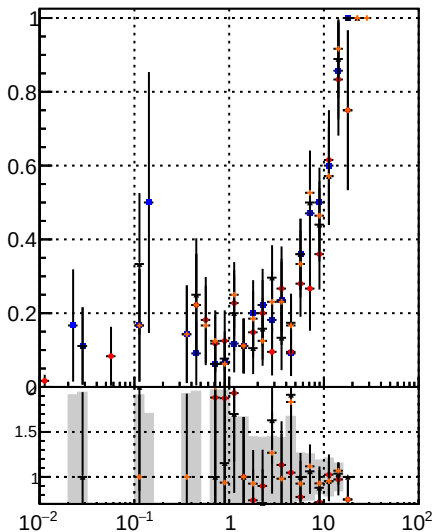
Fake rate vs vertpos Legend: DOM Displaced SUSY CKE (blue circles) DOM Displaced SUSY CKE fit (red circles) DOM Displaced SUSY mkFit BDT (orange circles)
