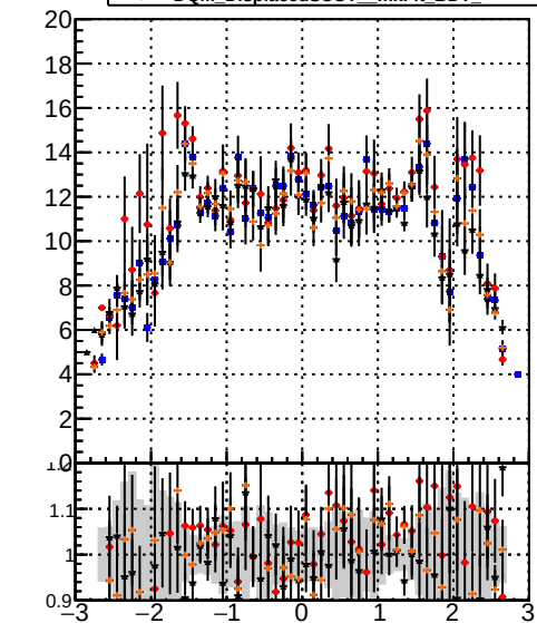
mean hit DQM_DisplacedSUSY_CKF DQM_DisplacedSUSY_mkFit DQM_DisplacedSUSY_CKF_BDT DQM_DisplacedSUSY_mkFit_BDT
