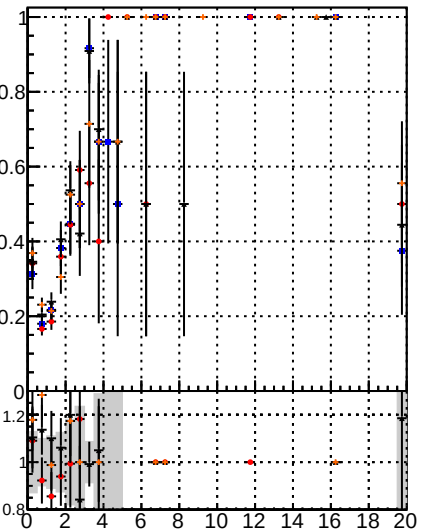
Fake rate vs. BSM Displaced SUSY CKFit BSM Displaced SUSY CKFit BDT
