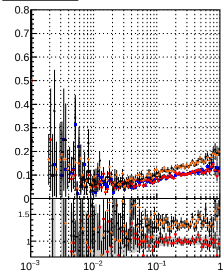
Fake rate vs DQM Displaced SUSY CKEFit DQM Displaced SUSY CKEFit DQM Displaced SUSY mkFit BDT
