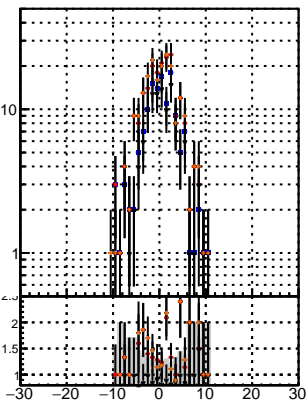
N of reco track vs dz
