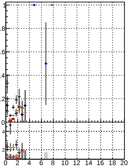
Fake rate vs. \chi^2 for BDT, BDT+CKE, and BDT+CKE+BDT
