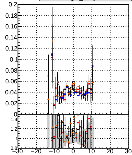
DOM Displaced SUSY CKE DOM Displaced SUSY CKEfit DOM Displaced SUSY BDT DOM Displaced SUSY CKEfit BDT
