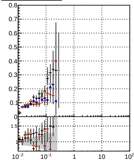
DOM Displaced SUSY CKE DOM Displaced SUSY CKEfit DOM Displaced SUSY BDT DOM Displaced SUSY CKEfit BDT
