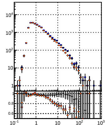
N of reco track vs p_T BQM Displaced SUSY GKEfit BQM Displaced SUSY MKFit BDT
