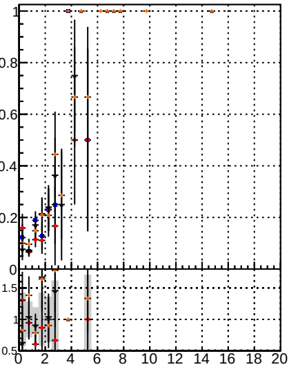
Fake rate vs. BDM Displaced SUSY CKE BDM Displaced SUSY CKE Fit BDM Displaced SUSY CKE Fit BDT
