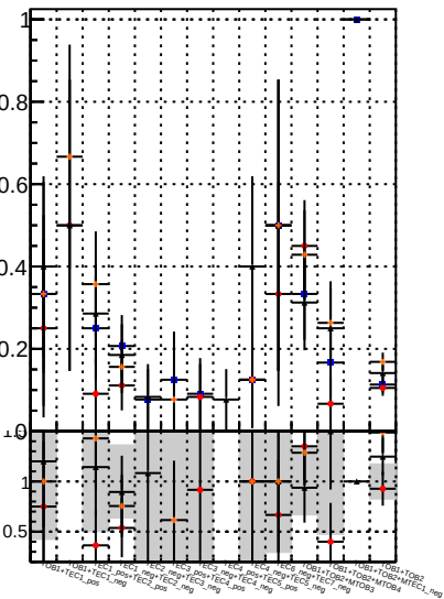
Fake rate vs. BDM Displaced SUSY CKE BDM Displaced SUSY CKE Fit BDM Displaced SUSY CKE Fit BDT
