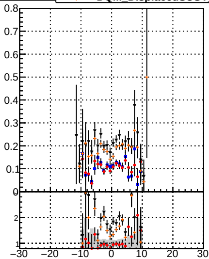
—•— DOM Displaced SUSY CKE —•— DOM Displaced SUSY CKEfit —•— DOM Displaced SUSY mkFit —•— DOM Displaced SUSY BDT
