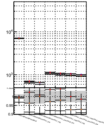
Legend for all plots: - Blue circle: BDM Displaced SUSY GKE - Red circle: BDM Displaced SUSY GKE - Orange circle: BDM Displaced SUSY GKE - Grey square: BDT - Black square: verSet
