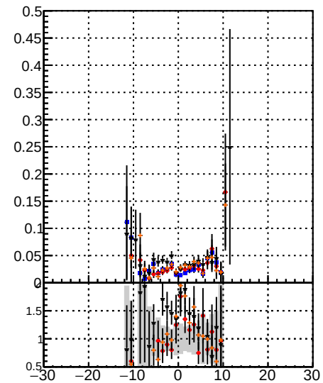
Fake rate vs d —●— BGM Displaced SUSY CKE Fit —●— BGM Displaced SUSY CKE Fit —●— BGM Displaced SUSY CKE Fit BDT
