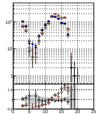
DOM Displaced SUSY CKE Displaced SUSY CKE mkt-fit BDT DOM Displaced SUSY CKE mkt-fit BDT
