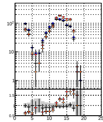
DOM Displaced SUSY CKE Displaced SUSY CKE mkt-fit BDT DOM Displaced SUSY CKE mkt-fit BDT
