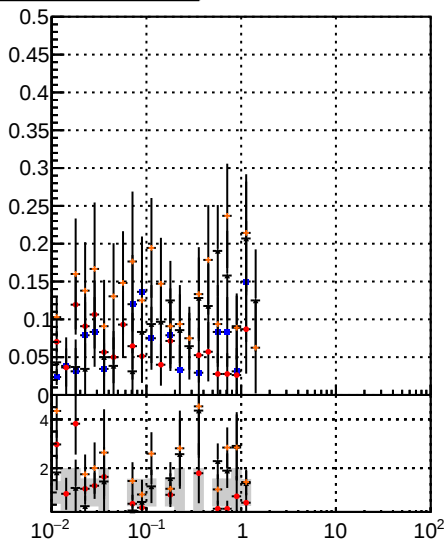
—•— DOM Displaced SUSY CKE —•— DOM Displaced SUSY CKE fit BDT —•— DOM Displaced SUSY mkt fit BDT
