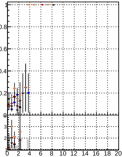
Fake rate vs. BDT Displaced SUSY CKFit BDT Displaced SUSY CKFit BDT
