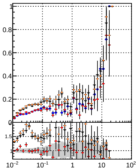
Fake rate vs v DOM Displaced SUSY CKE DOM Displaced SUSY CKEfit DOM Displaced SUSY BDT DOM Displaced SUSY mktfit BDT
