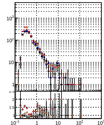
SUSY CKE SUSY mkFit SUSY CKE BDT SUSY mkFit BDT
