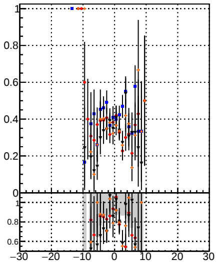
DOM Displaced SUSY CKEfit DOM Displaced SUSY mktfit DOM Displaced SUSY BDT
