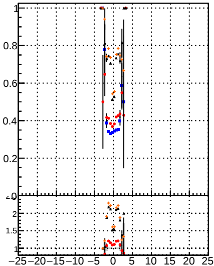
Fake rate vs d —●— BGM Displaced SUSY CKE Fit —●— BGM Displaced SUSY CKE Fit BDT —●— BGM Displaced SUSY CKE Fit BDT
