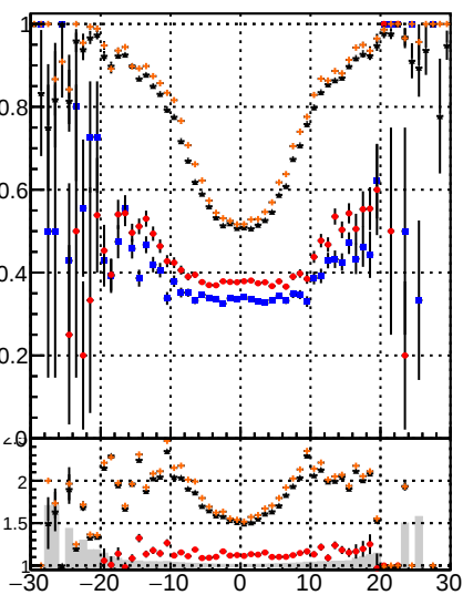
Fake rate vs d —●— BGM Displaced SUSY CKE Fit —●— BGM Displaced SUSY CKE Fit BDT —●— BGM Displaced SUSY CKE Fit BDT
