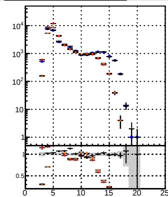
edSUSY—mkFit BDT
