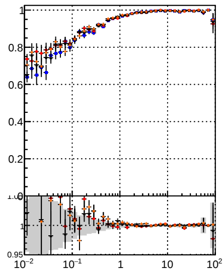
Fake rate vs v BDT Displaced SUSY CKE BDT Displaced SUSY CKE BDT Displaced SUSY mkFit BDT
