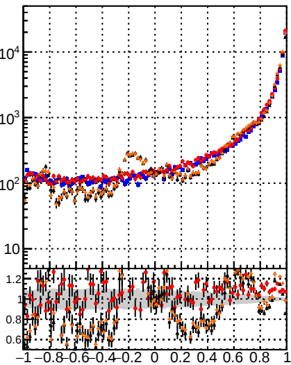
N of associated tracks (recoToSim) vs MVA1
