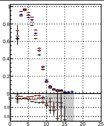
Fake rate vs la
